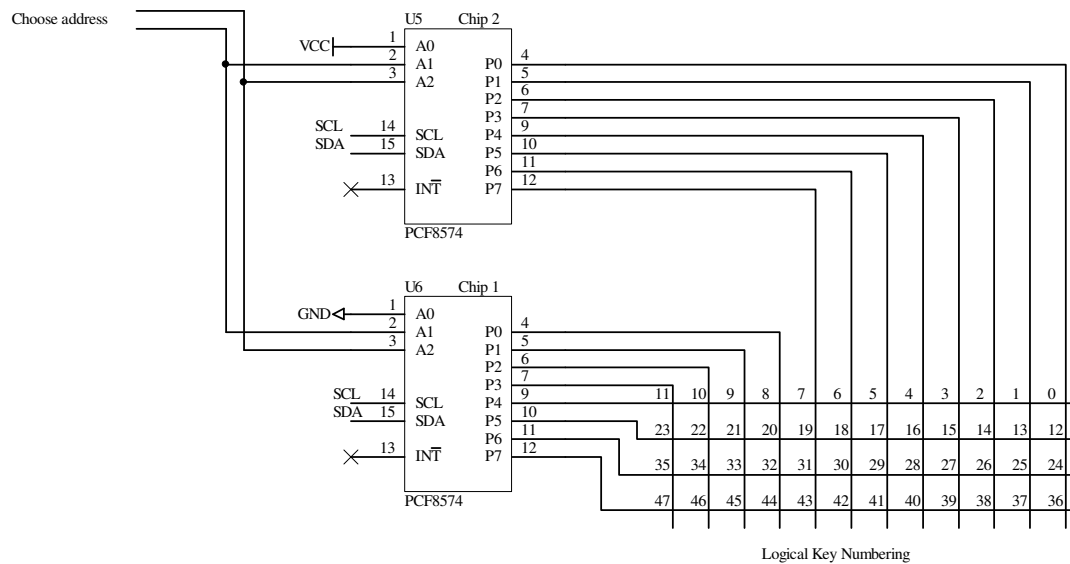
12 x 4 Keypad on an I2C Bus (Type 2)
