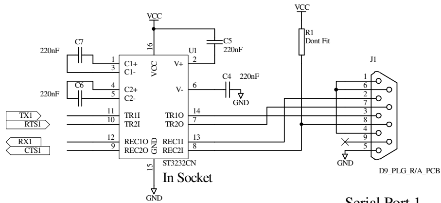
Serial Port 1
