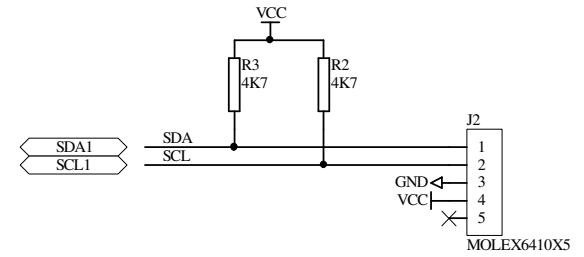
IIC Bus 1
